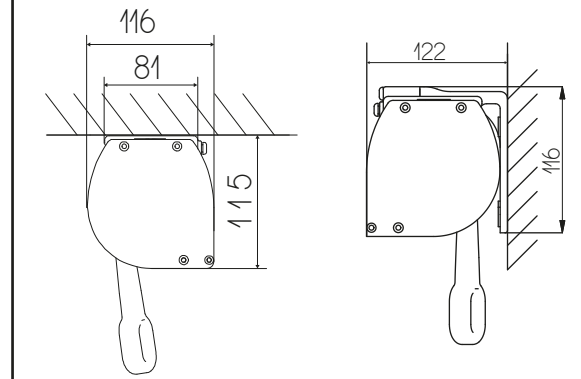
Encumbrances brackets with box
