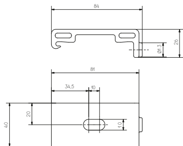
Ceiling brackets for Tb with box
