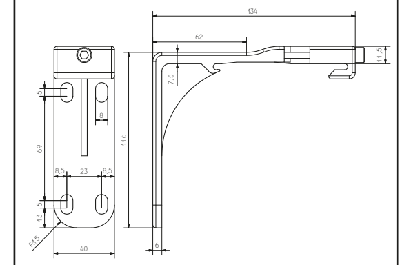
Wall brackets for Tb with box
