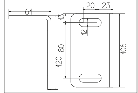
Brackets without box
